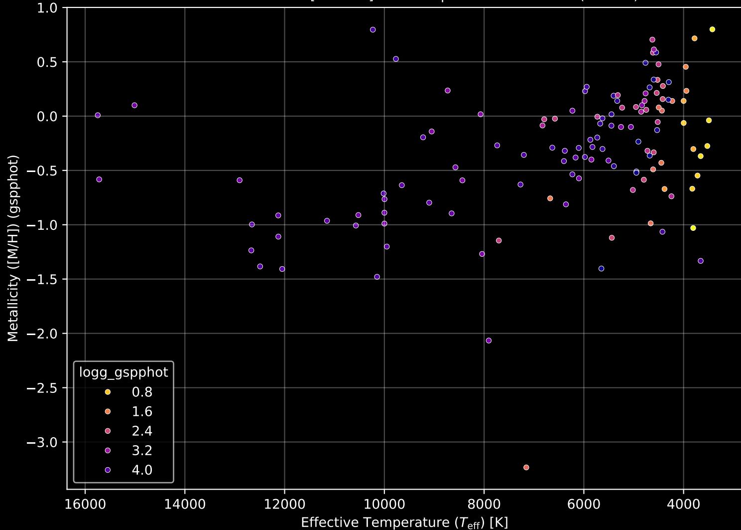
APOGEE DR17 Field: [079+00] Stellar Population Parameters (n= 126)
