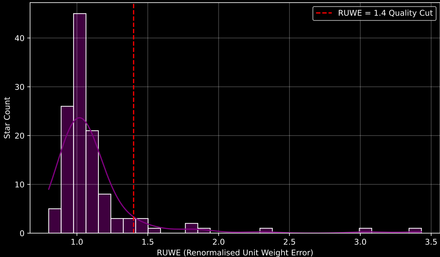
GAPOGEE DR17 Field [079+00] RUWE Distribution (n= 121)
