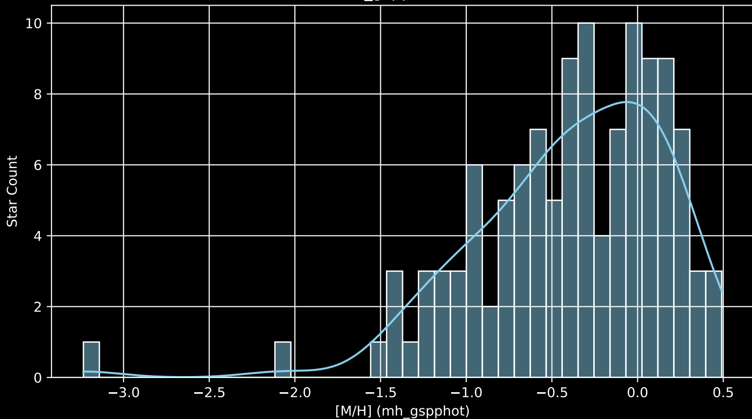
APOGEE DR17 Field: [079+00 [M/H] (mh_gspphot) (n= 118)
