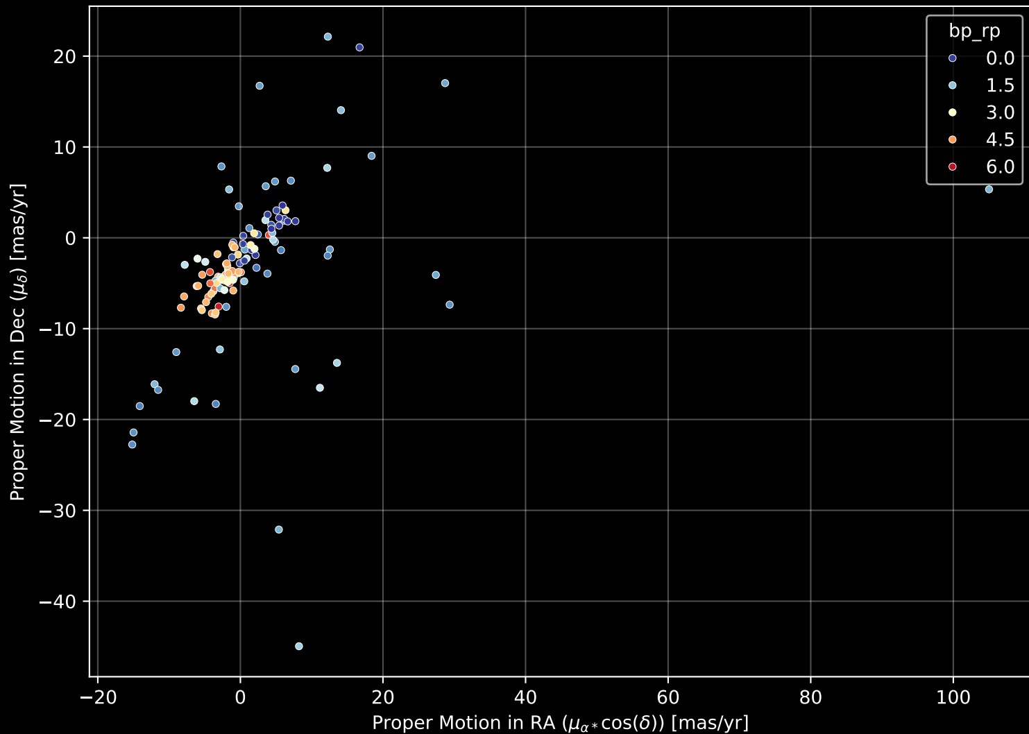
APOGEE DR17 Field: [079+00] Proper Motion Diagram (n= 126)
