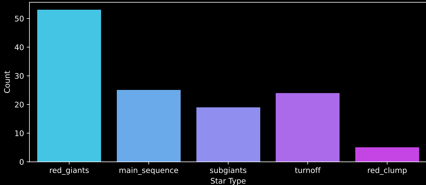
APOGEE DR17 Field: [079+00] Count plot of Star Type
