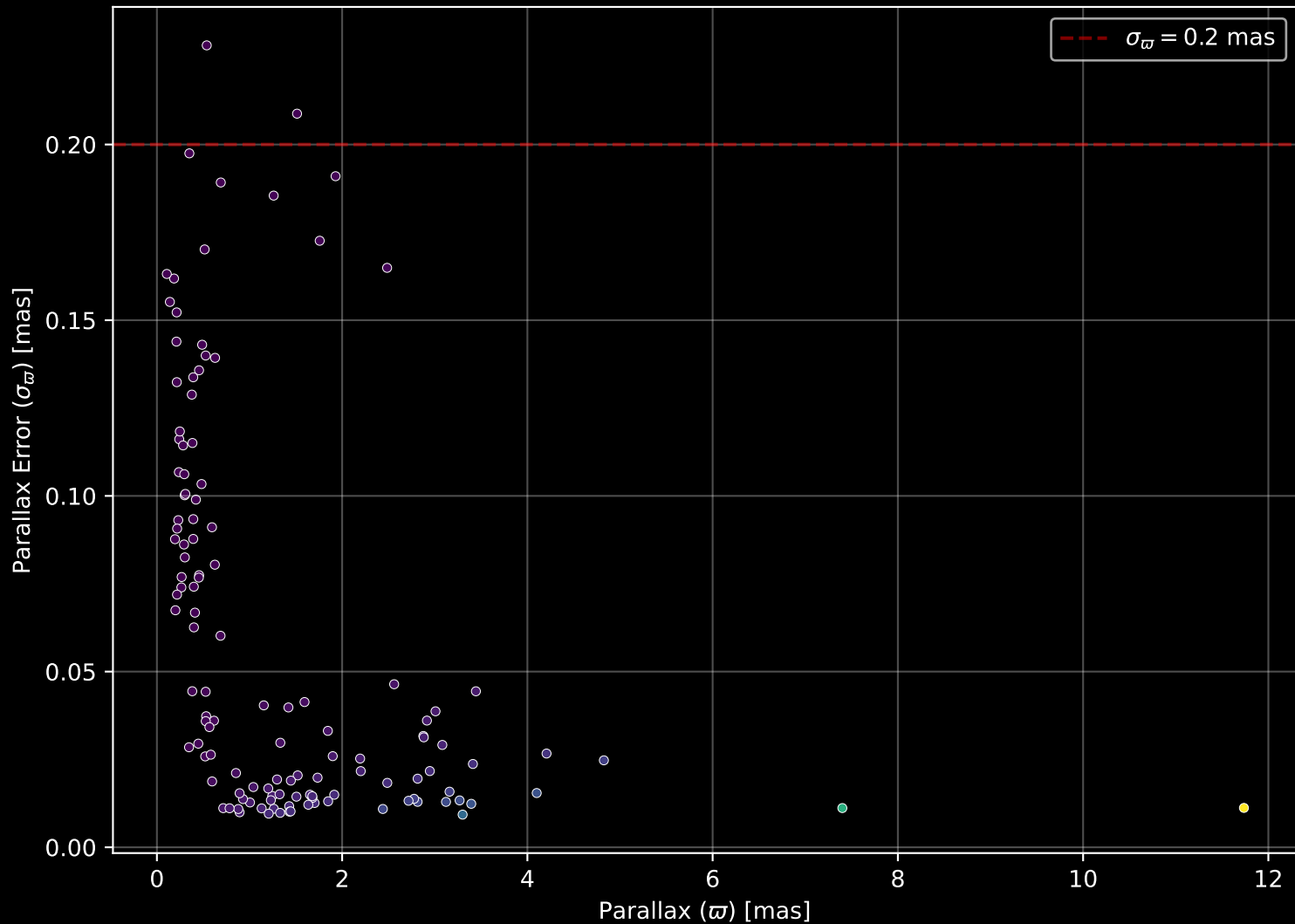
APOGEE DR17 Field: [079+00] Parallax Quality (n= 126)
